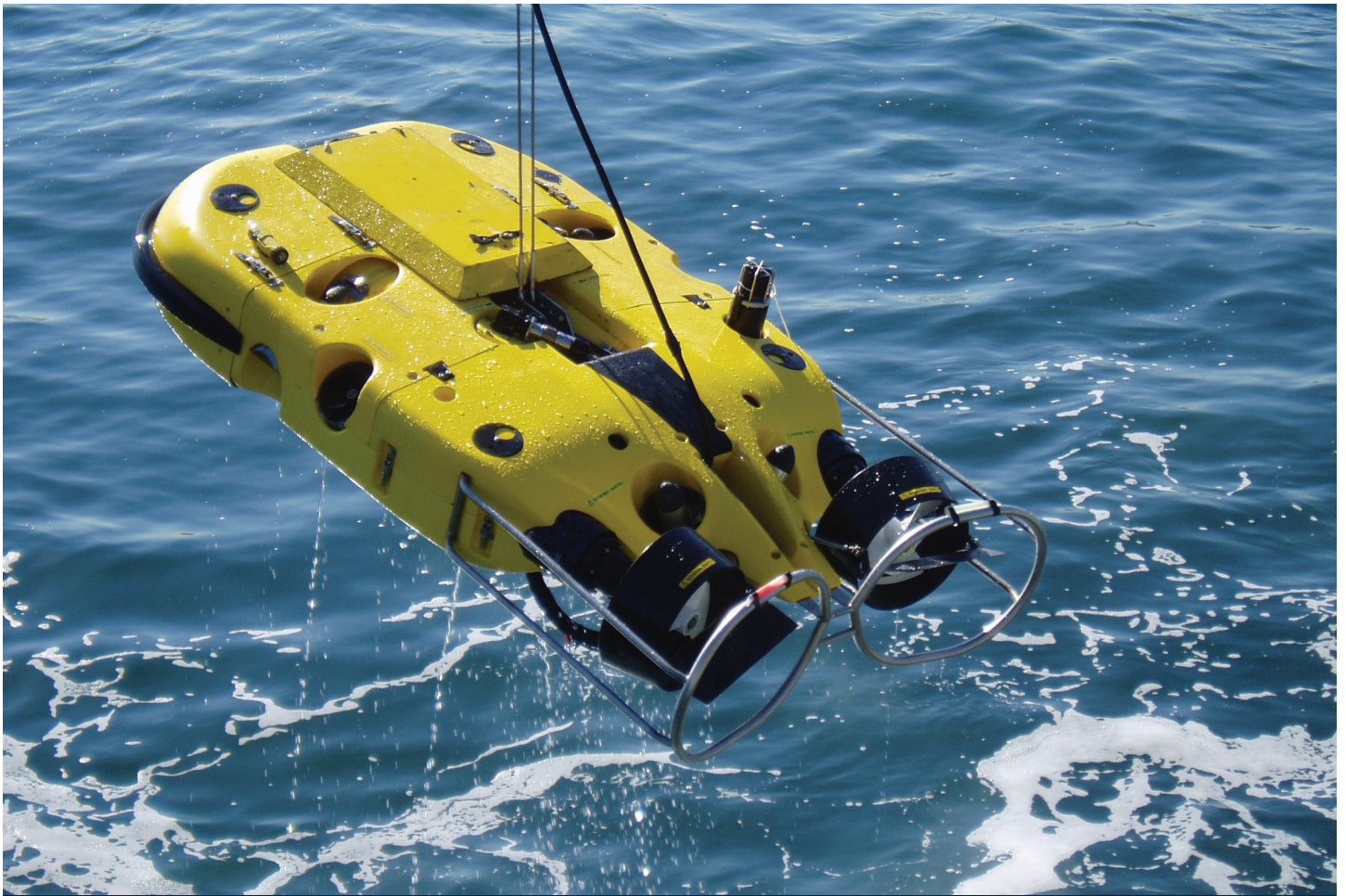
Saab Double Eagle MK II Mine Disposal Vehicle – Perfectly suited to operate in the strong currents and harsh conditions encountered in Australia.
